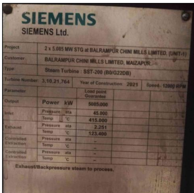
Figure 3: Nameplates of turbines within the plant
