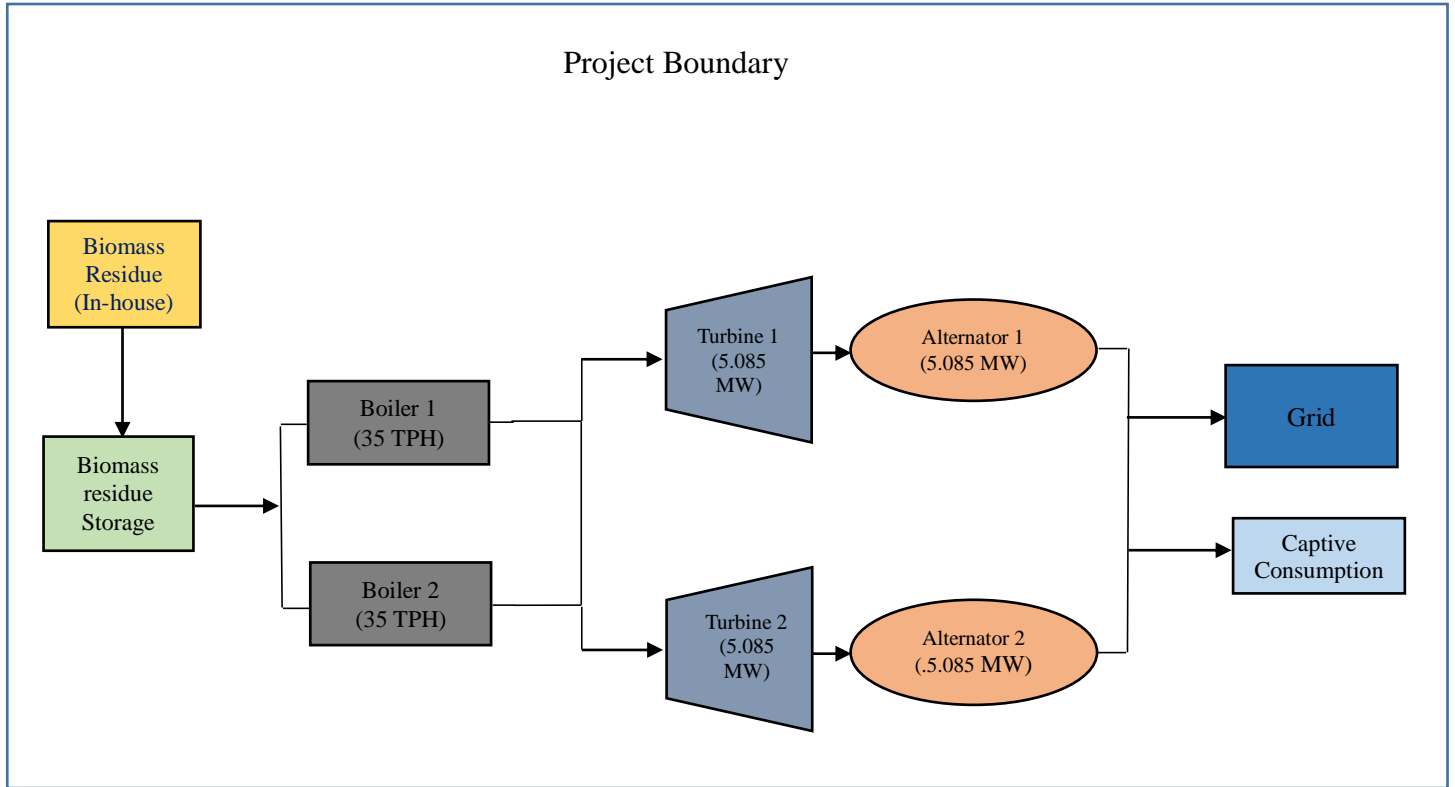
Figure 5: Schematic representation of project boundary
